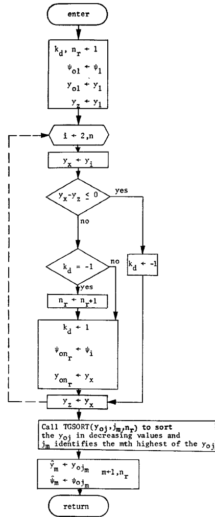
Fig. 3. Mathematical flow diagram of subroutine SELEC ( \phi^o, \psi_i, \hat{\psi}_m, k, n, n_r, \hat{y}_m ).
